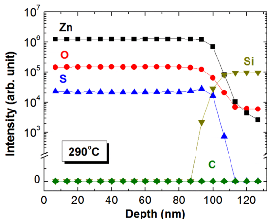
FIG. 1. Depth profile of Zn(O,S) with S/Zn=0.37, up to the Si substrate.
