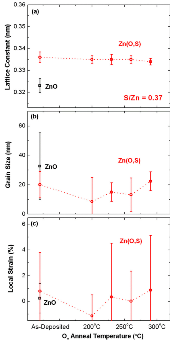
FIG. 5. Plots of (a) lattice constant, (b) grain size, and (c) local strain vs. O 2 annealing temperature for the as-deposited ZnO, as-deposited Zn(O,S) with S/Zn = 0.37, and Zn(O,S) with S/Zn = 0.37, oxygen annealed at different temperatures on quartz substrates.
