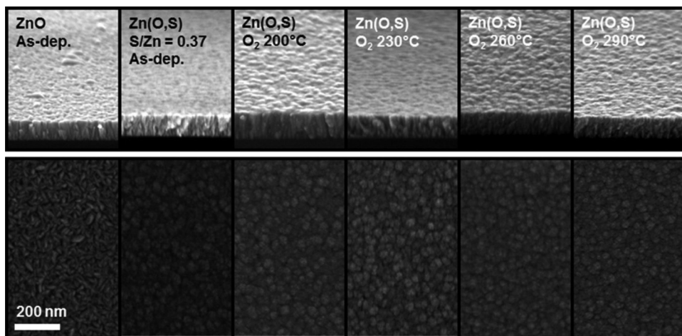
FIG. 6. Cross-sectional and plan-view FESEM images for the as-deposited ZnO, as-deposited Zn(O,S) with S/Zn = 0.37, and Zn(O,S) with S/Zn = 0.37, oxygen annealed at 200 °C, 230 °C, 260 °C, and 290 °C.
