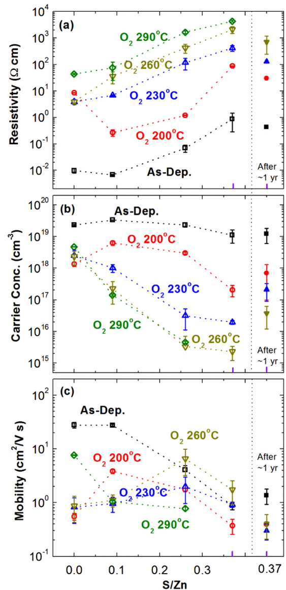
FIG. 2. Plots of (a) resistivity, (b) electron carrier concentration, and (c) electron mobility vs. S/Zn, for the as-deposited Zn(O,S) and Zn(O,S) samples annealed at 200 °C, 230 °C, 260 °C, and 290 °C in O 2 . Measurements were repeated for films after \sim 1 yr with S/Zn=0.37, as shown on the right side of the plots.
