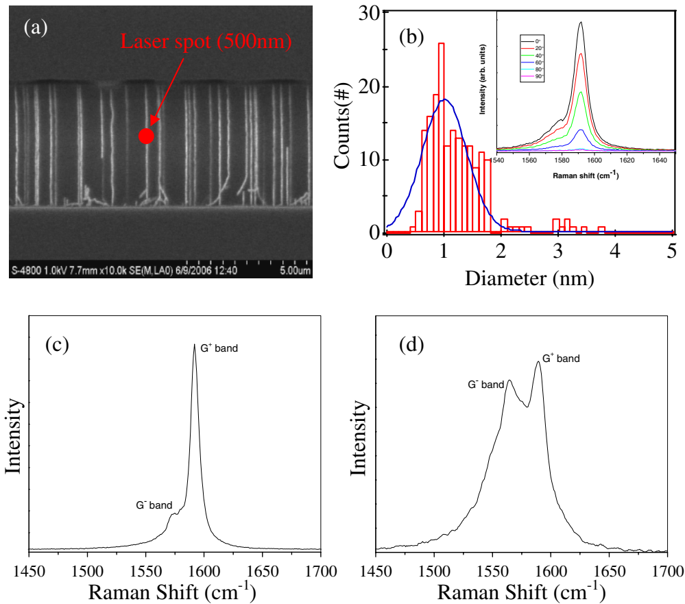
Fig. 1. (Color online) Detailed characterization of aligned carbon nanotubes. (a) SEM image of aligned nanotubes between source and drain electrodes, where the red dot stands for laser spot with 0.5 \mu\text{m} in diameter. (b) Histogram of diameter distribution of as-synthesized nanotubes. Inset: G band intensity as a function of the angle of polarization for an individual nanotube. (c) Typical Raman spectrum of semiconducting SWNTs characterized as Lorentzian lineshape. (d) Typical Raman spectrum of metallic SWNTs characterized as Breit-Wigner-Fano (BWF) lineshape.
