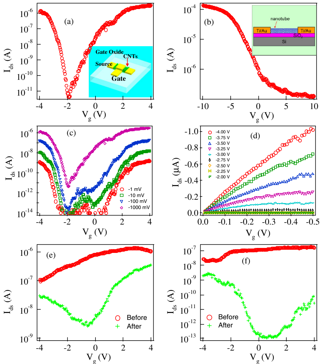
Fig. 3. (Color online) (a) I - V_g curve of a top-gated transistor exhibiting ambipolar behavior V_{ds} = -1 V. Inset: schematic diagram of device. (b) I - V_g curve of a back-gated transistor exhibiting p-type unipolar behavior V_{ds} = -1 V. Inset: schematic diagram of device. (c) A family of I - V_g curves at V_{ds} = -1, -10, -100, -1000 mV. (d) A family of I - V_{ds} curves at different gate voltages. (e, f) I - V_g curves for predominantly p- and n-type device, respectively.
