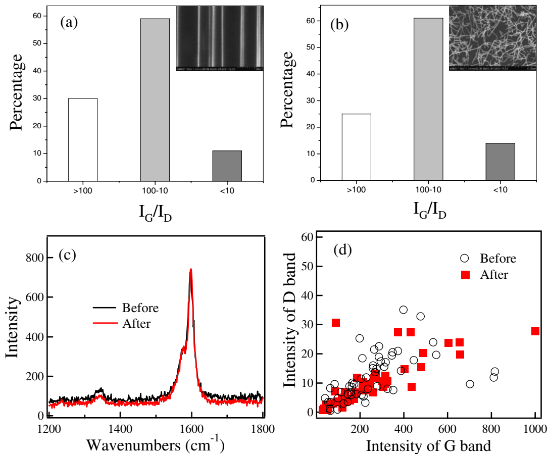
Fig. 2. (Color online) Defect analysis for aligned nanotubes on quartz (a) and randomly grown nanotubes on Si/SiO 2 (b). (c) Raman spectra of a nanotube before (black) and after (red) transfer, showing little difference. (d) Raman intensity of D- and G-bands of an ensemble of 60 nanotubes before and after transfer.
