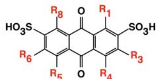
Extended Data Table 1 | AQDS screened by theoretical calculations
