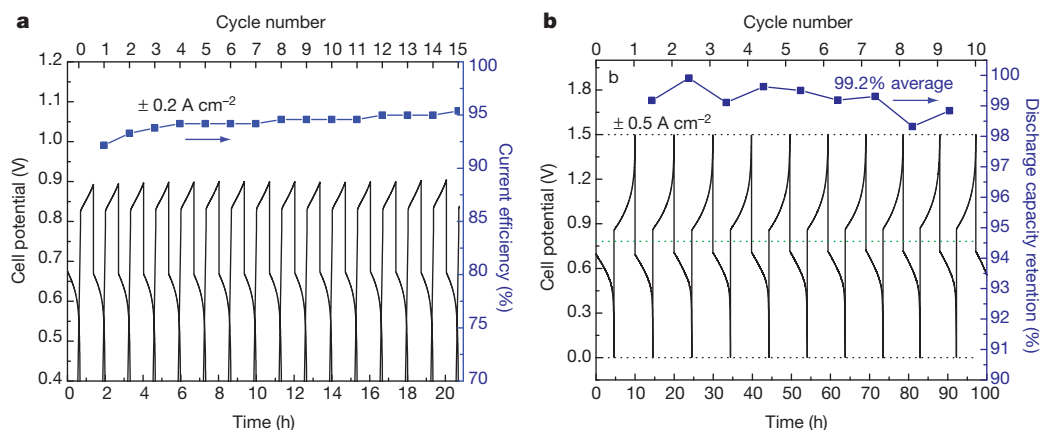
Figure 2 | Cell cycling behaviour. a , Constant-current cycling at 0.2\text{ A cm}^{-2} at 40^\circ\text{C} using a 2\text{ M HBr} + 0.5\text{ M Br}_2 solution on the positive side and a 0.1\text{ M AQDS} + 2\text{ M H}_2\text{SO}_4 solution on the negative side; current efficiency is indicated for each complete cycle. b , Constant-current cycling at 0.5\text{ A cm}^{-2}
