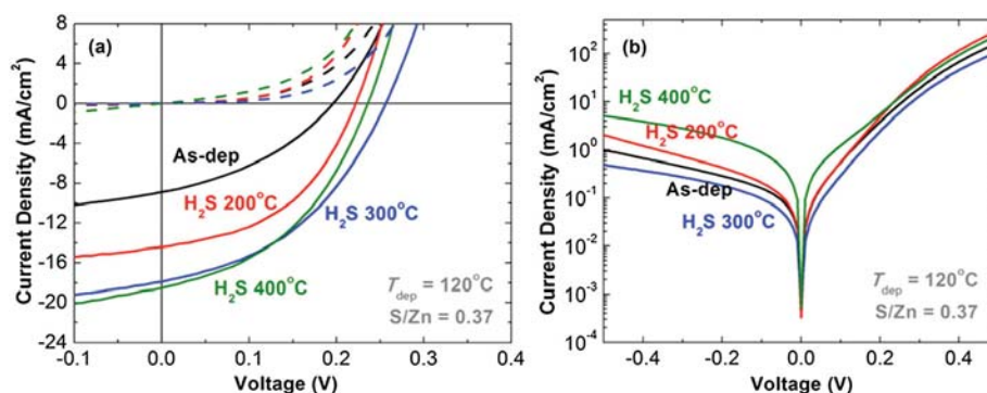
Figure 4. (Color) (a) Current density vs. voltage ( J - V ) plots under dark (dotted) and 1 Sun illumination (solid) and (b) semilog J - V plots under dark for devices with the SnS layer annealed at different temperatures having Zn(O,S), S/Zn = 0.37 as the buffer layer.
