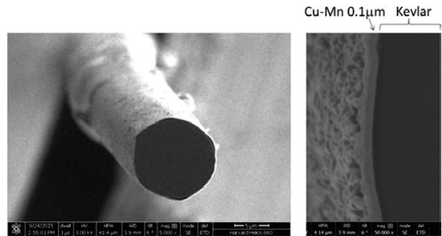
Fig. 7. SEM of a Kevlar fiber 11 μm in diameter coated with 0.1 μm CVD copper-manganese alloy. On the right, a closer view of the Cu-Mn coating.
