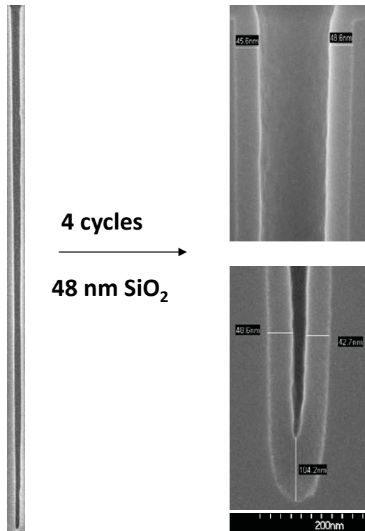
Fig. 3. ALD of alumina-doped silica as an insulator for TSVs [3].
