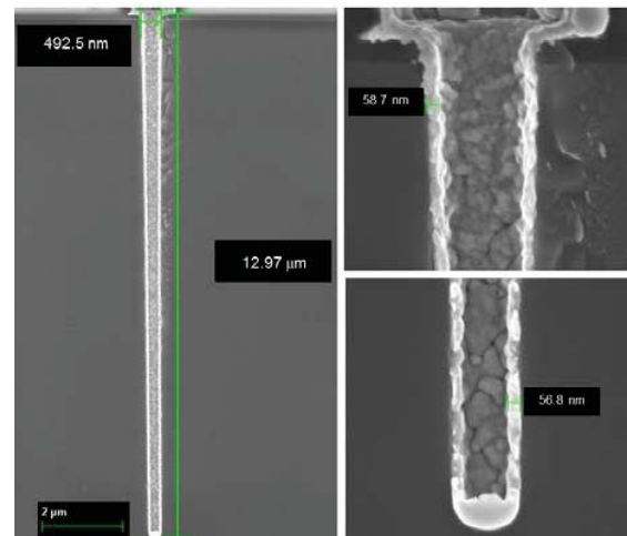
Fig. 5. CVD copper layer inside a narrow, high-aspect ratio hole [4].
