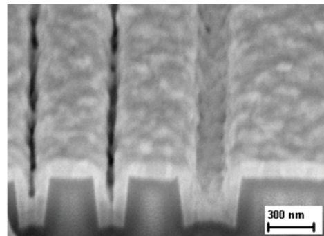
Fig. 1. Bottom-up growth by iodine-catalyzed CVD of copper-manganese alloy [2].
