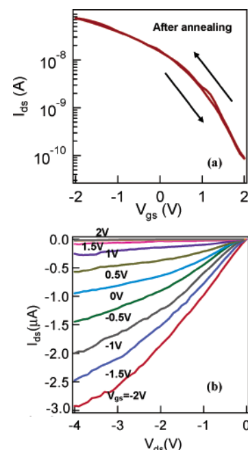
Figure 3. p-type GeNW FETs characteristics after removal of surface oxide by annealing in a vacuum at \sim 450 °C. (a) Current versus gate voltage ( I_{\text{ds}} - V_{\text{gs}} ) curves showing nearly eliminated hysteresis after annealing (measured in a vacuum) of the same device as in Figure 2. The bias voltage used to record this curve was V_{\text{ds}} = 100 mV. (b) Current versus voltage ( I_{\text{ds}} - V_{\text{ds}} ) curves under various gate voltages as labeled.
