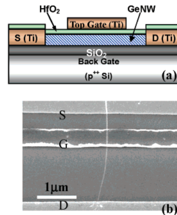
Figure 9. Top-gated p-type GeNW FETs with high- \kappa HfO 2 dielectrics. (a) A schematic side view of the device. (b) A top-view SEM image of the device. SEM acceleration voltage = 5 keV. (c) I_{\text{ds}}-V_{\text{gs}} characteristics of a typical device exhibiting little hysteresis ( V_{\text{ds}} = 100 mV).
