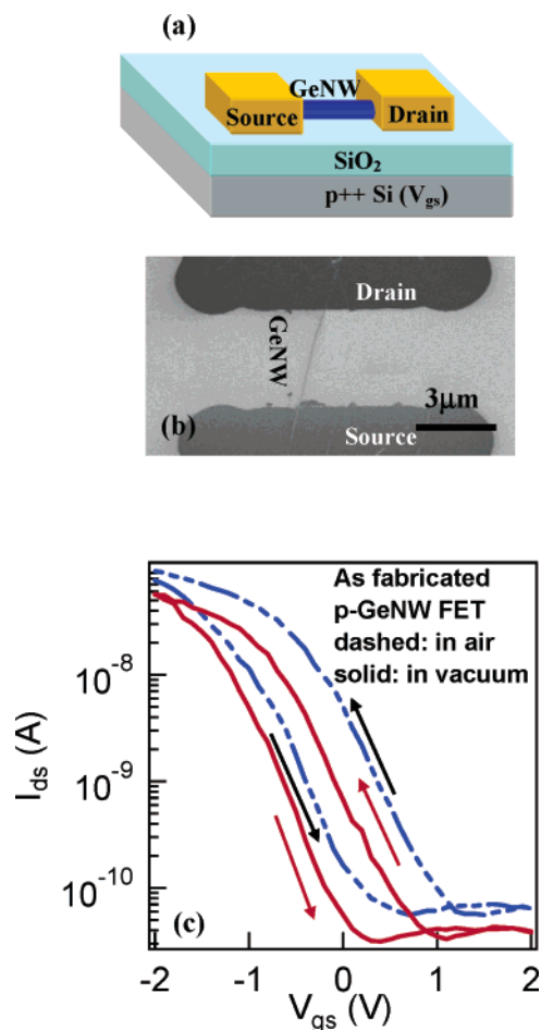
Figure 2. Back-gated p-type GeNW FETs. (a) A schematic view of the device structure. The SiO 2 thickness is t_{\text{ox}} = 10 nm. The doped Si substrate is used for the back-gate. (b) A SEM top-view image of an individual GeNW device recorded at an acceleration voltage of 5 keV. The electrodes and GeNW appear dark under this imaging condition because they conduct electrons better than the SiO 2 background. (c) A typical as-fabricated unpassivated GeNW FET exhibiting large hysteresis under back-and-forth gate sweeping (direction marked by arrows, V_{\text{ds}} = 100 mV) measured with the device placed in air and in a vacuum ( 5 \times 10^{-7} Torr), respectively.
