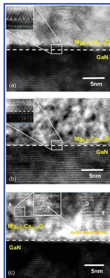
Figure 2. Cross-sectional TEM of \text{Mg}_x\text{Ca}_{1-x}\text{O} films grown on GaN(0001) surface. (a) \text{Mg}_{0.25}\text{Ca}_{0.75}\text{O}/\text{GaN} ; (b) \text{Mg}_{0.51}\text{Ca}_{0.49}\text{O}/\text{GaN} ; (c) \text{Mg}_{0.72}\text{Ca}_{0.28}\text{O}/\text{GaN} ; grain boundaries can be found between each region labeled with letters. The enlarged grain boundary between region A and B shows both darkness contrast as well as pattern difference. Region B is showing a three line repeating pattern, which indicates two different orientation grains are overlapping together. A similar pattern can also be found in regions D and E.
