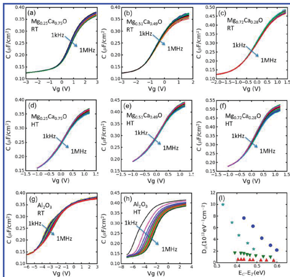
Figure 4. C - V measurements for Mg_xCa_{1-x}O/GaN and Al_2O_3/GaN samples. The frequency ranges of all samples are from 1 kHz to 1 MHz. (a) 20 °C Al_2O_3(5\text{ nm})/Mg_{0.25}Ca_{0.75}O(15\text{ nm})/GaN ; (b) 20 °C Al_2O_3(5\text{ nm})/Mg_{0.51}Ca_{0.49}O(15\text{ nm})/GaN ; (c) 20 °C Al_2O_3(5\text{ nm})/Mg_{0.72}Ca_{0.28}O(15\text{ nm})/GaN ; (d) 150 °C Al_2O_3(5\text{ nm})/Mg_{0.25}Ca_{0.75}O(15\text{ nm})/GaN ; (e) 150 °C Al_2O_3(5\text{ nm})/Mg_{0.51}Ca_{0.49}O(15\text{ nm})/GaN ; (f) 150 °C Al_2O_3(5\text{ nm})/Mg_{0.72}Ca_{0.28}O(15\text{ nm})/GaN ; (g) 20 °C Al_2O_3(20\text{ nm})/GaN for comparison; (h) 150 °C Al_2O_3(20\text{ nm})/GaN . (i) D_{it} summary of four samples determined by the conductance method: Al_2O_3(20\text{ nm})/GaN (light blue star), Al_2O_3(5\text{ nm})/Mg_{0.72}Ca_{0.28}O(15\text{ nm})/GaN (blue circles), Al_2O_3(5\text{ nm})/Mg_{0.51}Ca_{0.49}O(15\text{ nm})/GaN (green down triangle), and Al_2O_3(5\text{ nm})/Mg_{0.25}Ca_{0.75}O(15\text{ nm})/GaN (red up triangles).
