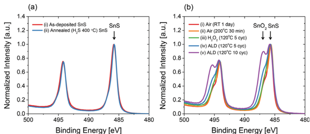
Figure 8. Normalized XPS spectra (Sn 3d) of a-i) as-deposited and a-ii) annealed SnS films (400 °C in H 2 S) and b) annealed SnS films (400 °C in H 2 S) with a SnO 2 layer formed via b-i) an ambient air exposure at room temperature for 1 day, b-ii) annealing in 10 Torr of air at 200 °C for 30 min, b-iii) an exposure to 5 cycles of 7.5 Torr s H 2 O 2 vapor at 120 °C, and b-iv) 5 and b-v) 10 cycles of ALD at 120 °C, respectively.
